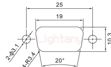
面板开孔 (Panel Cutout)
