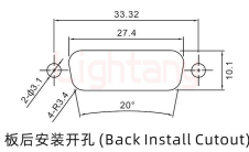
板后安装开孔 (Back Install Cutout)
