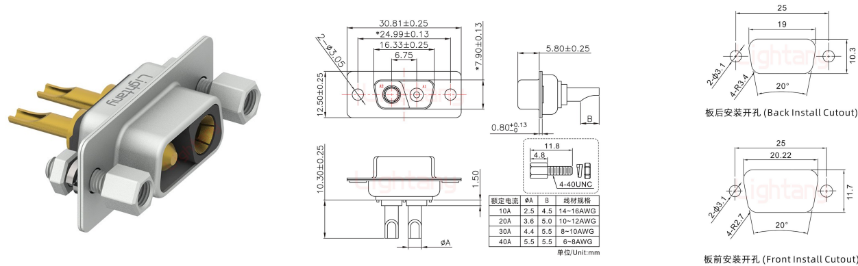
板前安装开孔 (Front Install Cutout)
