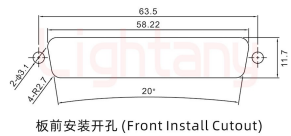
板前安装开孔 (Front Install Cutout)
