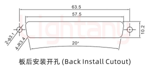
板后安装开孔 (Back Install Cutout)
